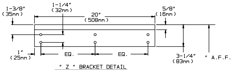
" Z " BRACKET DETAIL
